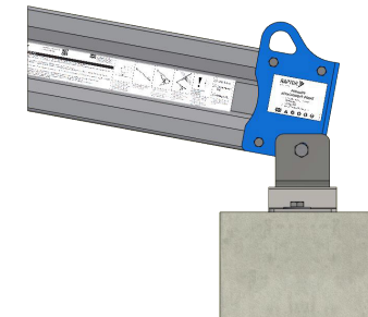
REAR ATTACHMENT - CONCRETE FLOOR MOUNT
